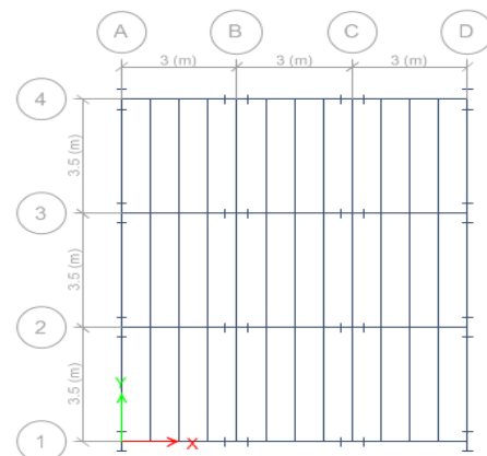
Figure 3.1 Plan of the building
