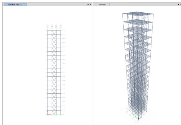
Figure 3.4 Elevation and 3D view of the building with V bracings at center bay
