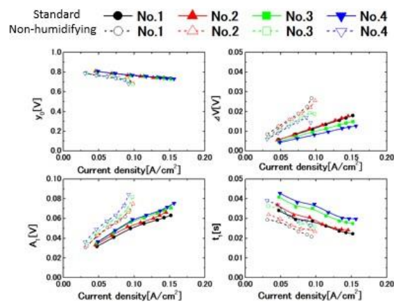
Figure 11. Polarization distribution obtained by the conventional diagnostics
