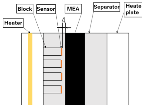
Figure 5. Cross diagram of PEFC
